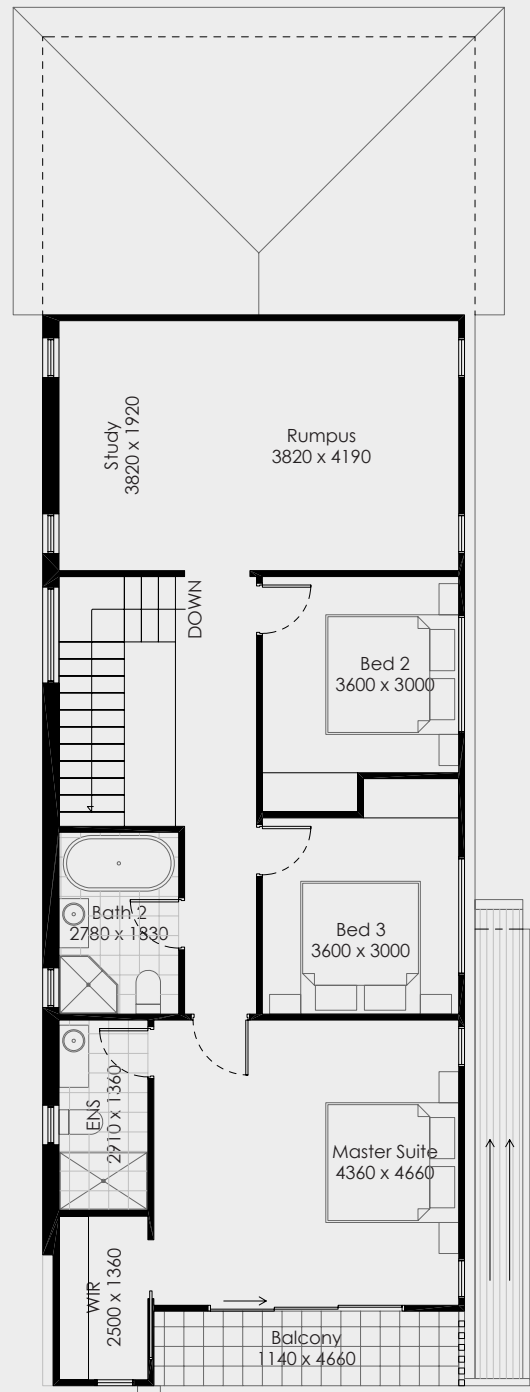
First Floor
