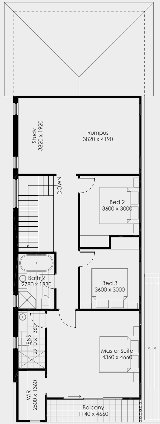
First Floor
